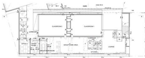
A-03 DOMUS GALDIUM 2TH FLOOR 26.4.2021 BUREAU ARCHITECTS OY
